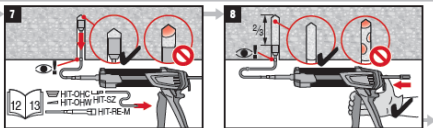
FIGURE 9A—MANUFACTURER'S PRINTED INSTALLATION INSTRUCTIONS (MPII) (Cont)
